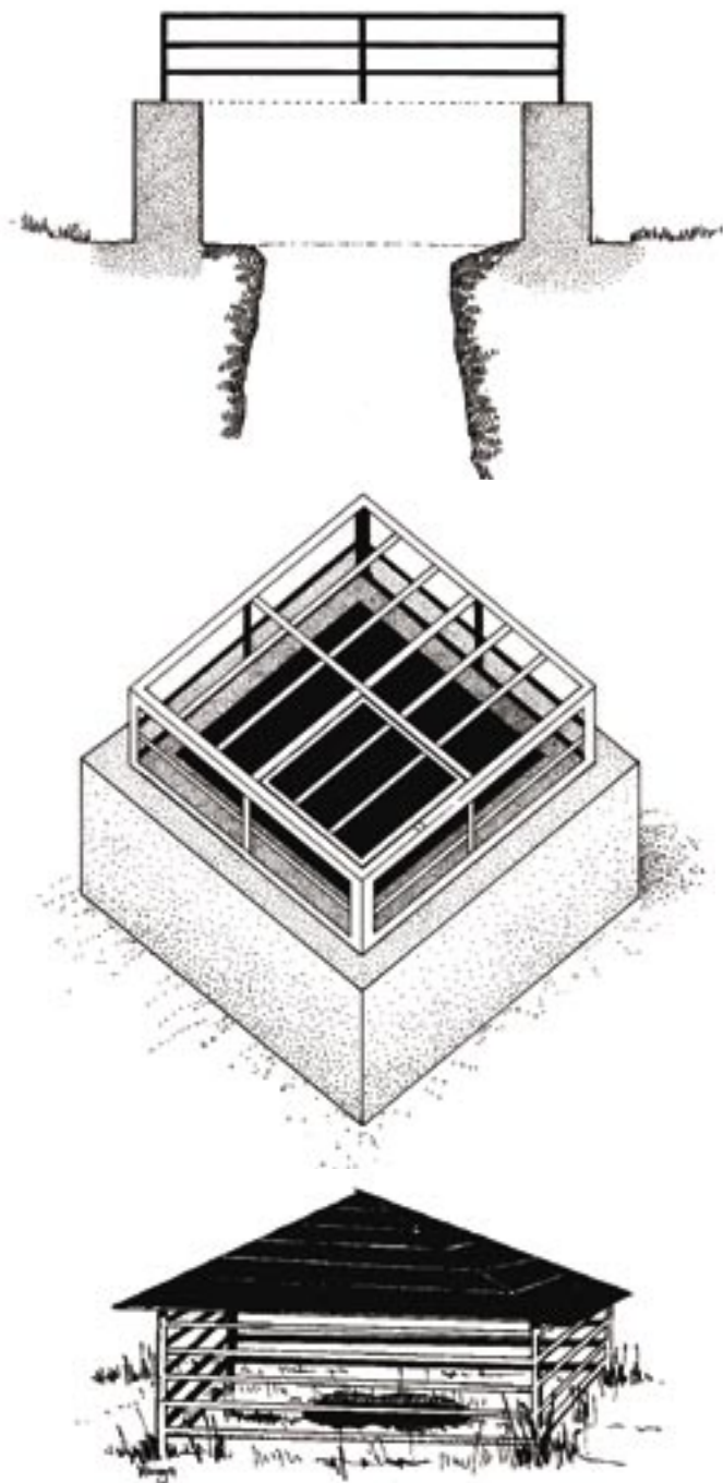
Figure 7. Grilles for vertical shafts. Horizontal grilles close to the ground should be avoided as these create safety problems and can be blocked by vegetation. Stabilisation of the top of the cave or shaft may be needed. Bats seem to have no difficulty flying up vertical shafts and then through a vertical grille.
